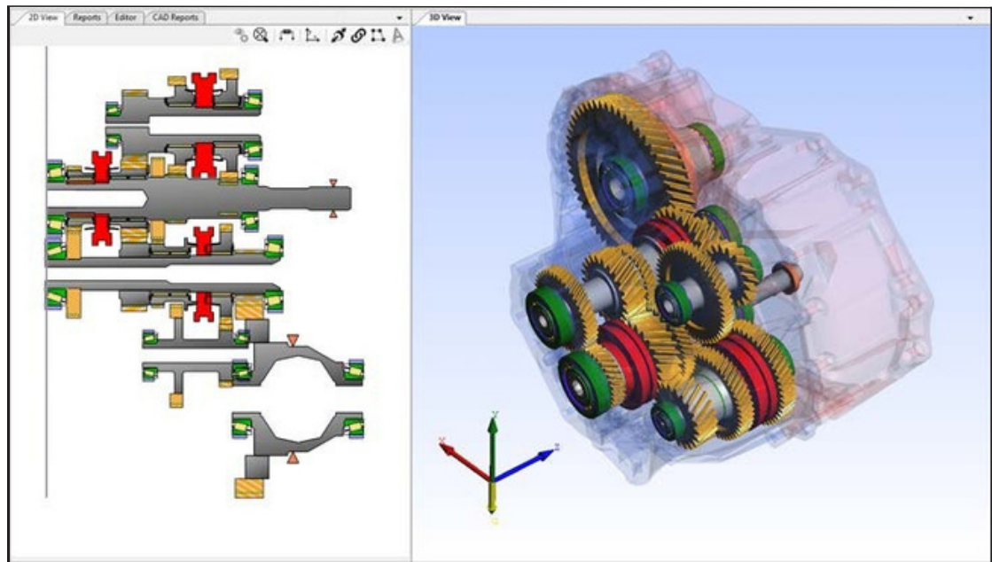
Figure 2 System-level transmission simulation model.
