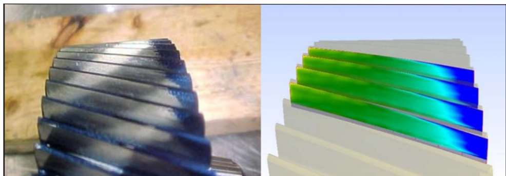
Figure 5 Measured and simulated loaded contact patterns.
