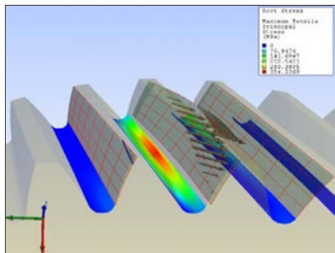
Figure 4 Hybrid FE and Hertzian-based loaded tooth contact analysis.
